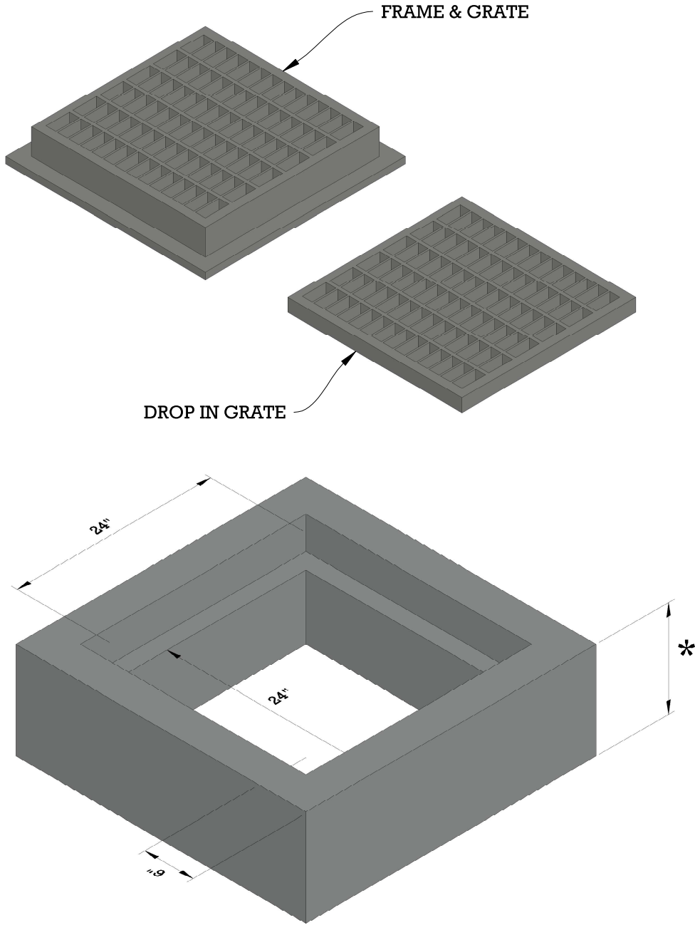
ISOMETRIC VIEW
