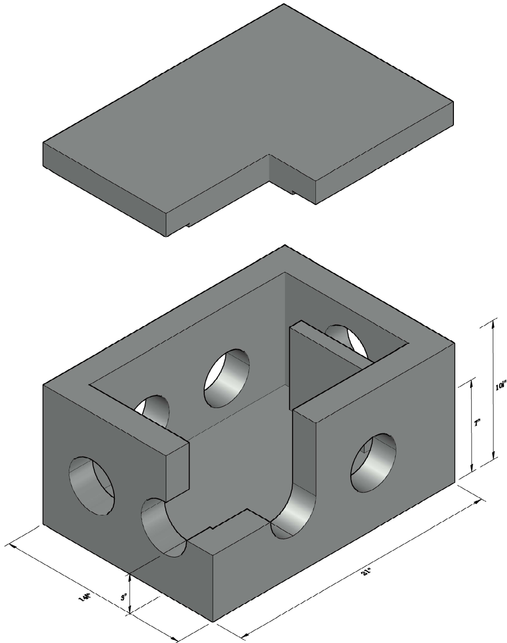
ISOMETRIC VIEW
