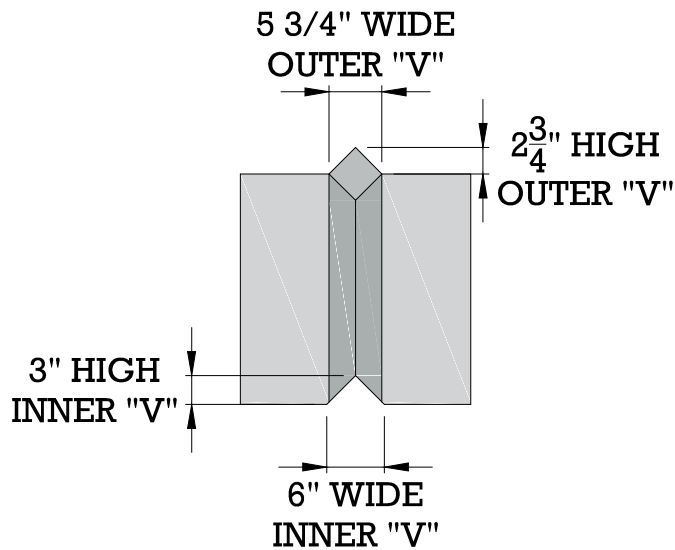
END VIEW
