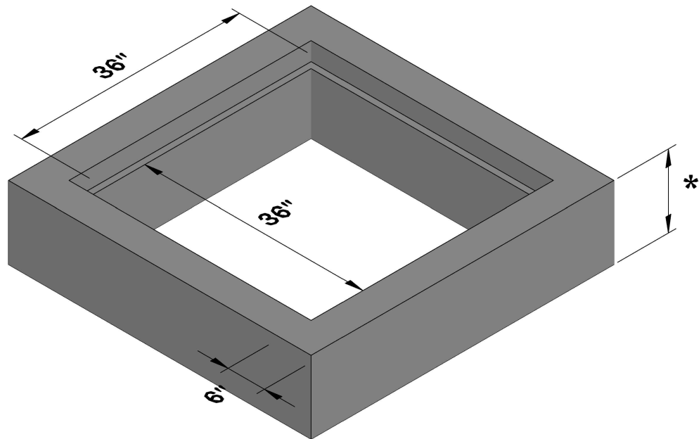
ISOMETRIC VIEW
