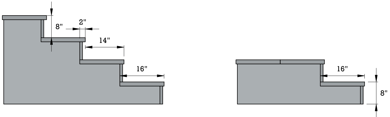
SIDE VIEW
